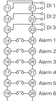
Alarm unit (option)
