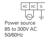
Power terminal
