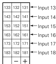
Input terminal 3
